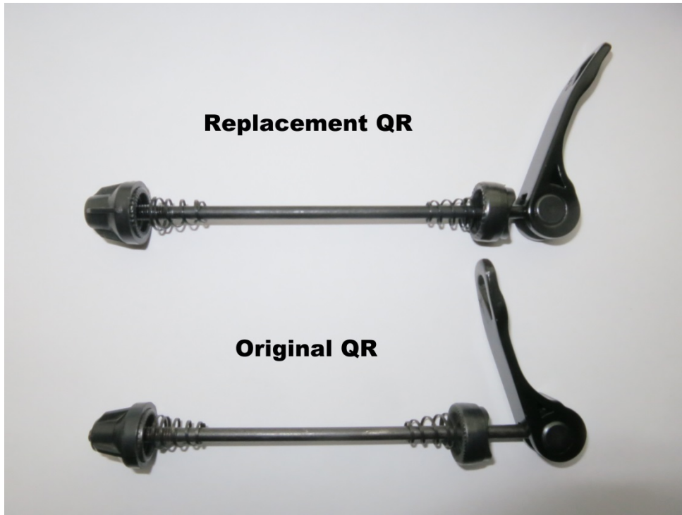
Quick release lever in open position
